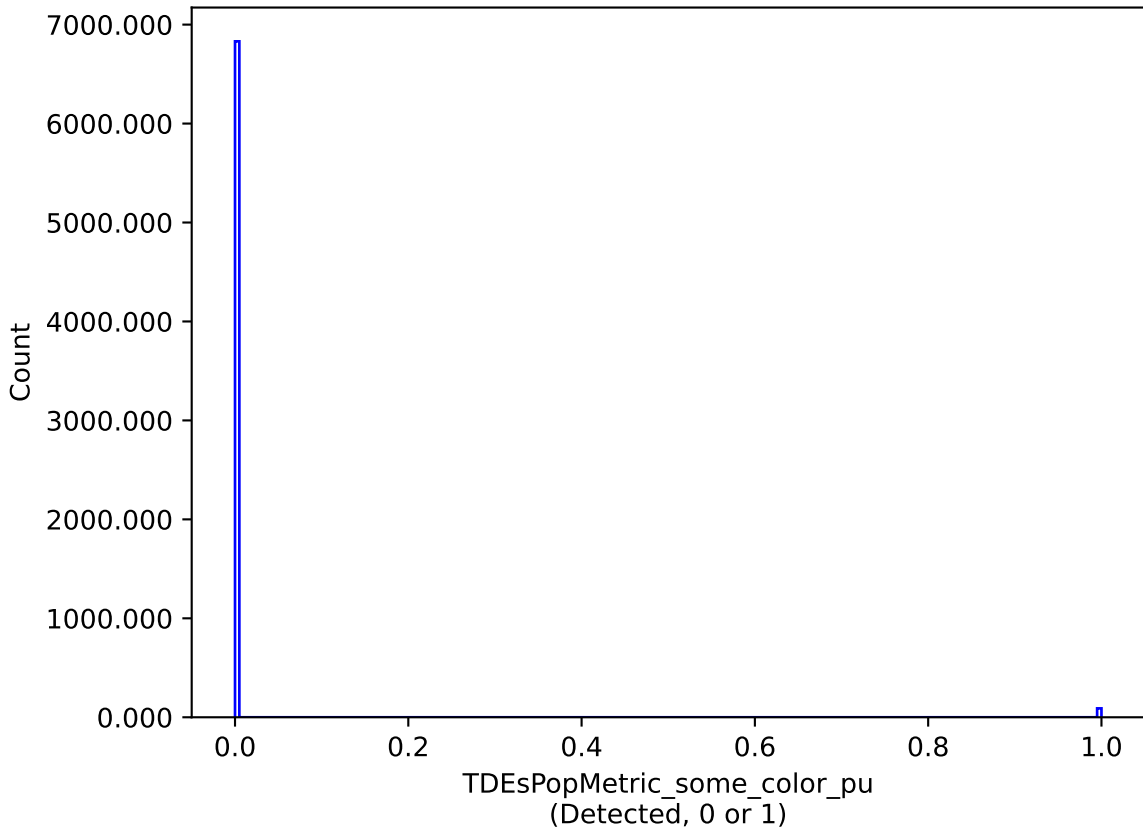
smc_lmc_v3.3_10yrs : TDEsPopMetric_some_color_pu
