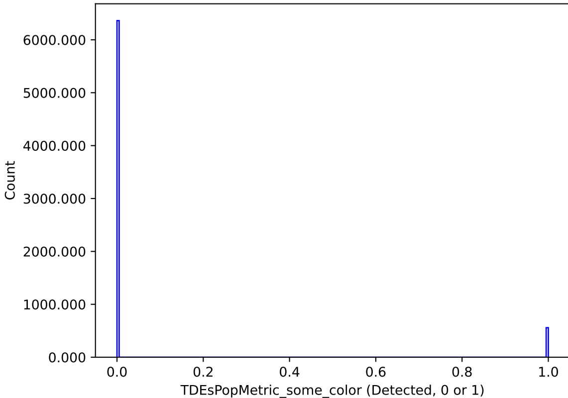
smc_lmc_v3.3_10yrs : TDEsPopMetric_some_color
