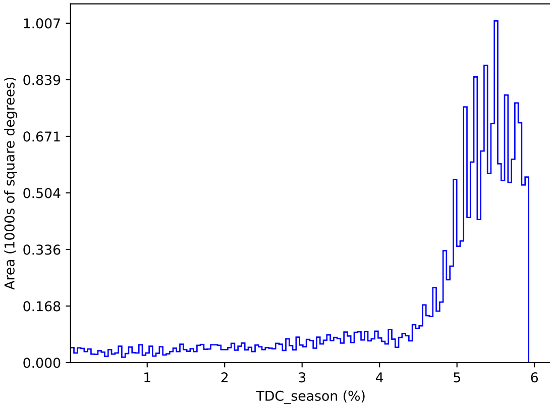
smc_lmc_v3.3_10yrs : TDC_season
