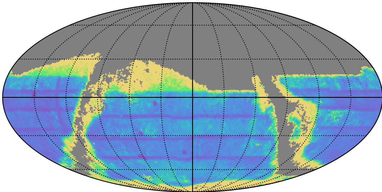
smc_lmc_v3.3_10yrs : TDC_precision
