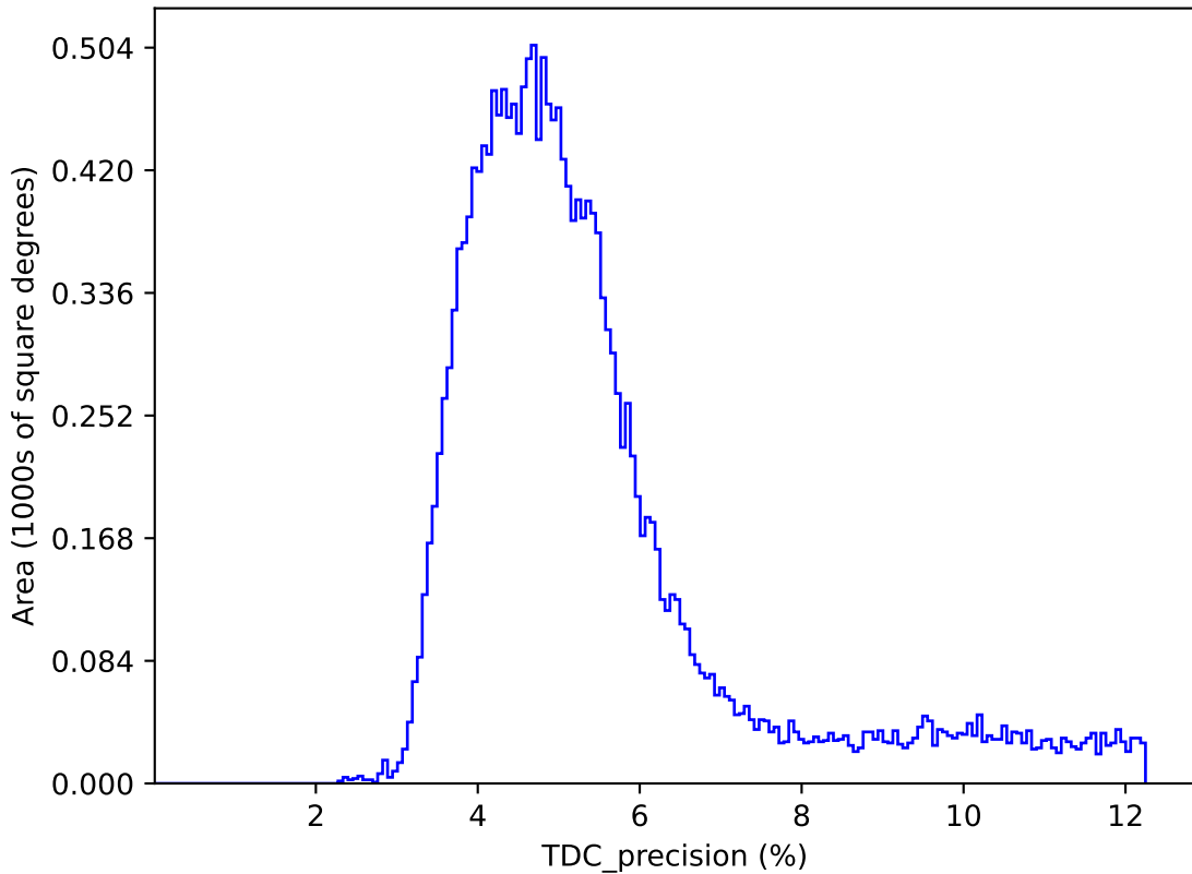
smc_lmc_v3.3_10yrs : TDC_precision
