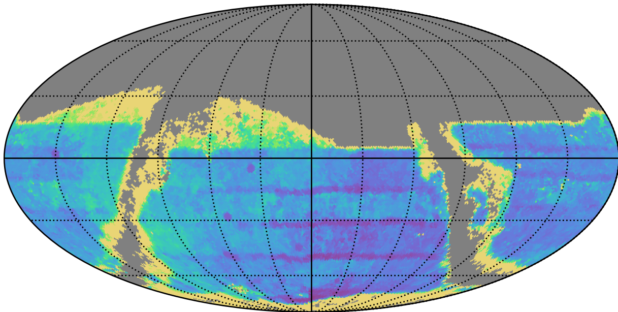
smc_lmc_v3.3_10yrs : TDC_accuracy
