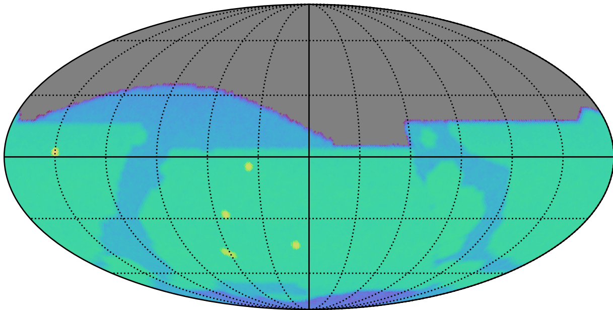
smc_lmc_v3.3_10yrs z: SurfaceBrightLimit
