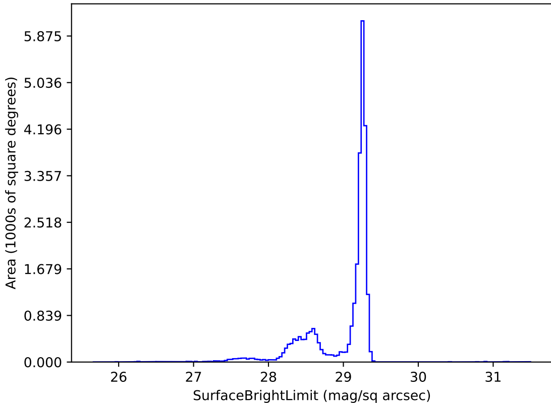
smc_lmc_v3.3_10yrs z: SurfaceBrightLimit
