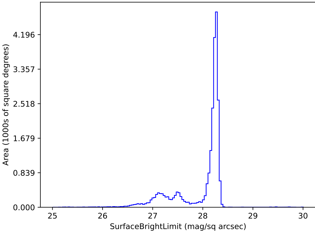
smc_lmc_v3.3_10yrs y: SurfaceBrightLimit
