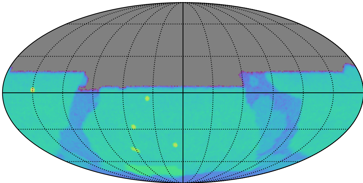
smc_lmc_v3.3_10yrs u: SurfaceBrightLimit
