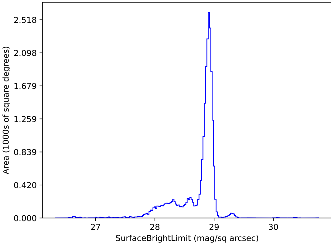
smc_lmc_v3.3_10yrs u: SurfaceBrightLimit
