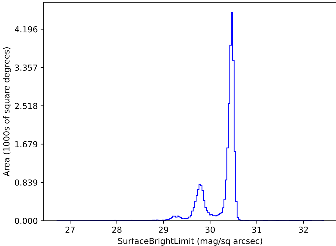
smc_lmc_v3.3_10yrs r: SurfaceBrightLimit
