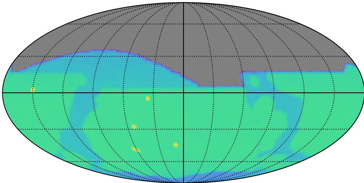
smc_lmc_v3.3_10yrs i: SurfaceBrightLimit
