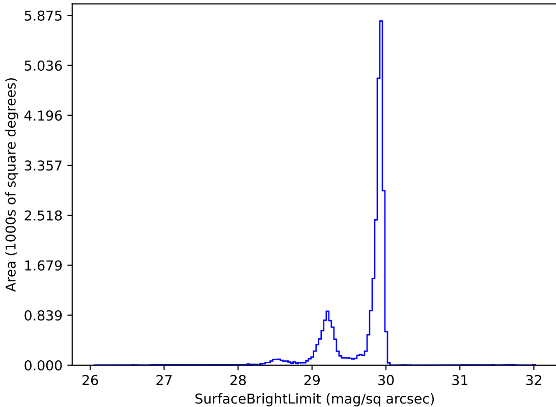
smc_lmc_v3.3_10yrs i: SurfaceBrightLimit
