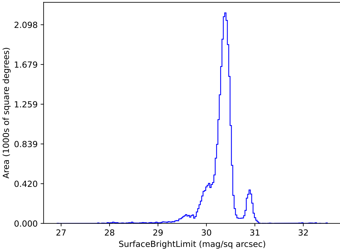
smc_lmc_v3.3_10yrs g: SurfaceBrightLimit
