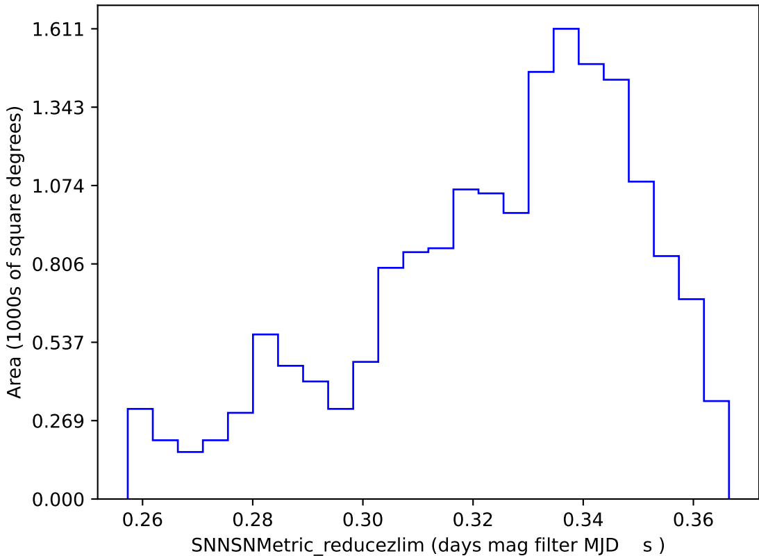
smc_lmc_v3.3_10yrs DDF excluded: SNNSNMetric_reducezlim
