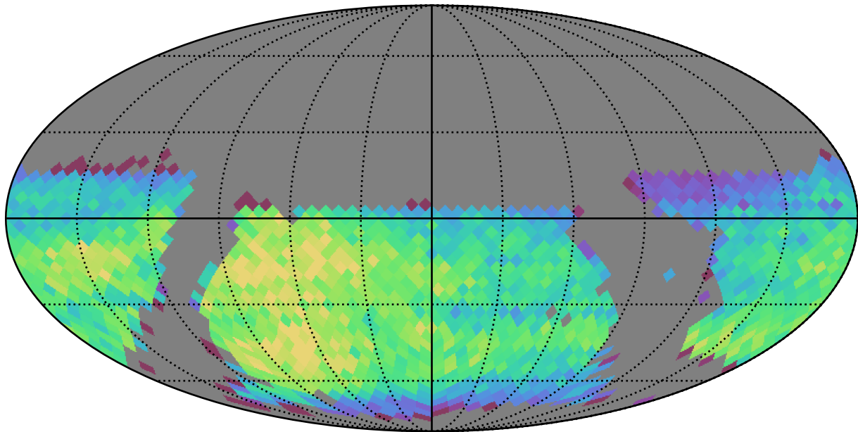
smc_lmc_v3.3_10yrs DDF excluded: SNNSNMetric_reducen_sn
