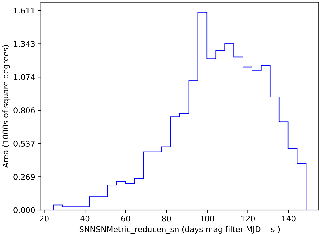
smc_lmc_v3.3_10yrs DDF excluded: SNNSNMetric_reducen_sn
