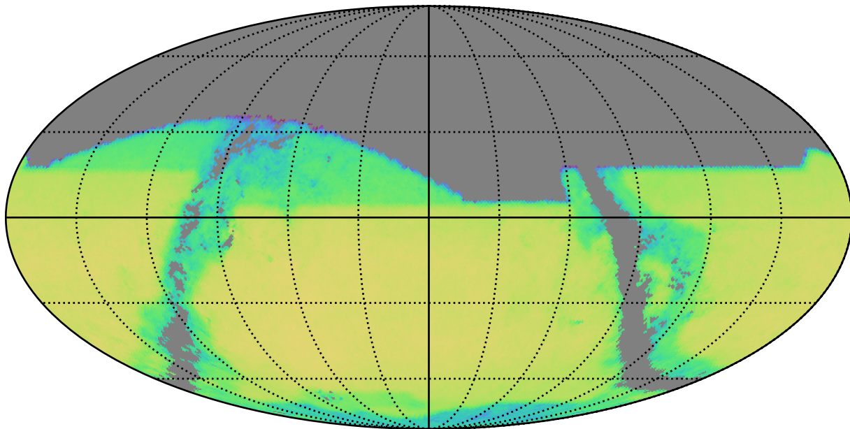
smc_lmc_v3.3_10yrs z band and non-DD: QSONumberCountsMetric
