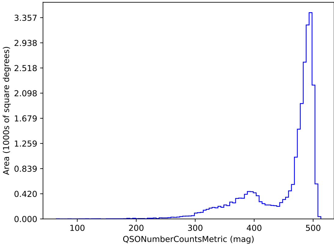
smc_lmc_v3.3_10yrs z band and non-DD: QSONumberCountsMetric
