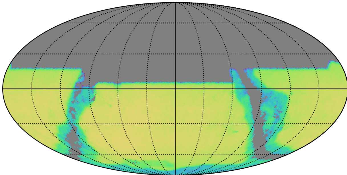
smc_lmc_v3.3_10yrs y band and non-DD: QSONumberCountsMetric
