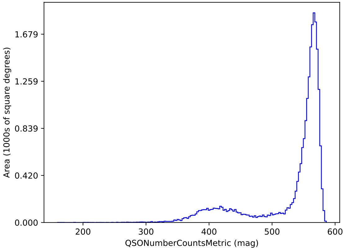
smc_lmc_v3.3_10yrs y band and non-DD: QSONumberCountsMetric
