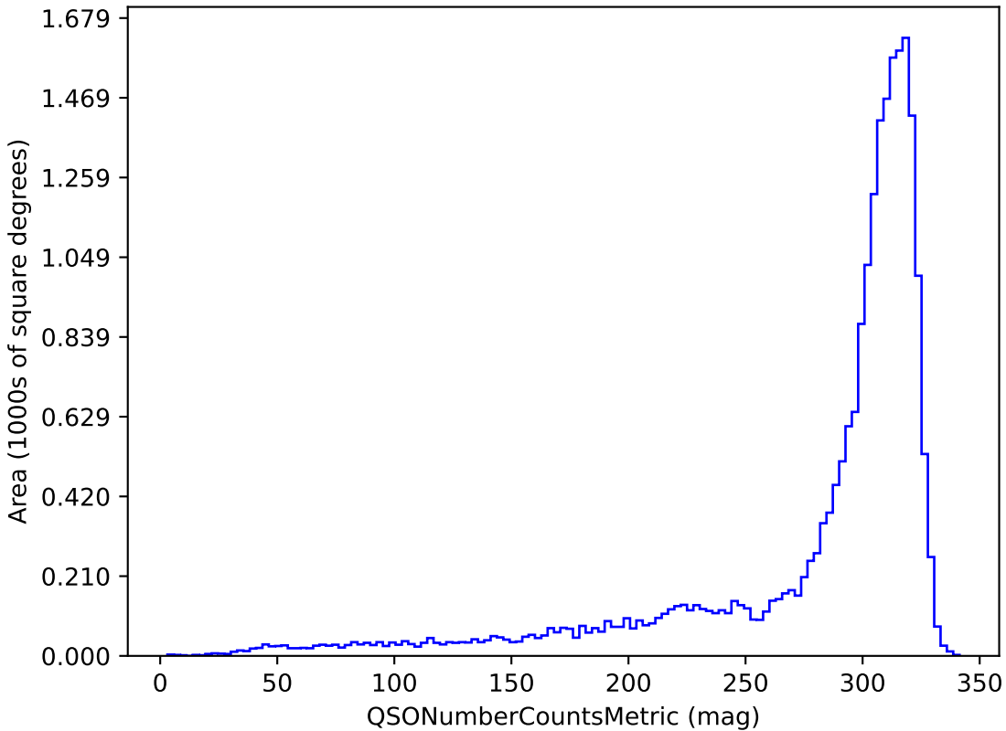
smc_lmc_v3.3_10yrs u band and non-DD: QSONumberCountsMetric
