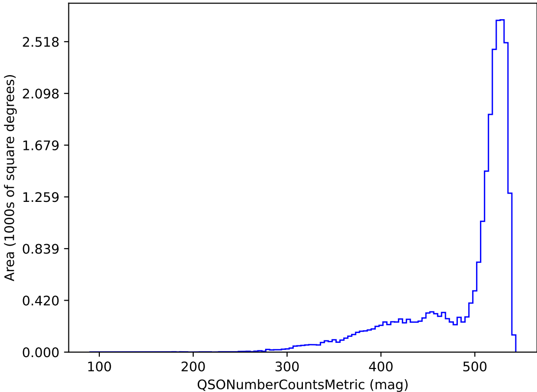
smc_lmc_v3.3_10yrs r band and non-DD: QSONumberCountsMetric
