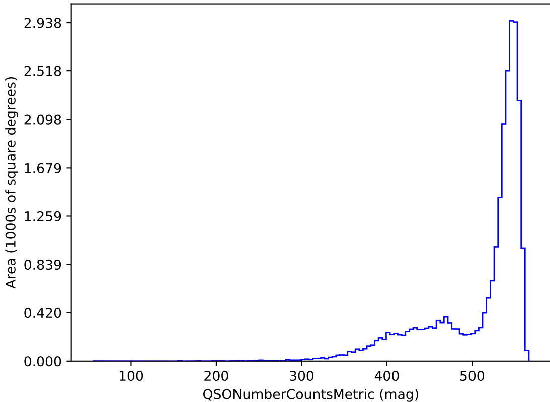
smc_lmc_v3.3_10yrs i band and non-DD: QSONumberCountsMetric
