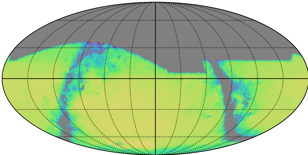
smc_lmc_v3.3_10yrs g band and non-DD: QSONumberCountsMetric
