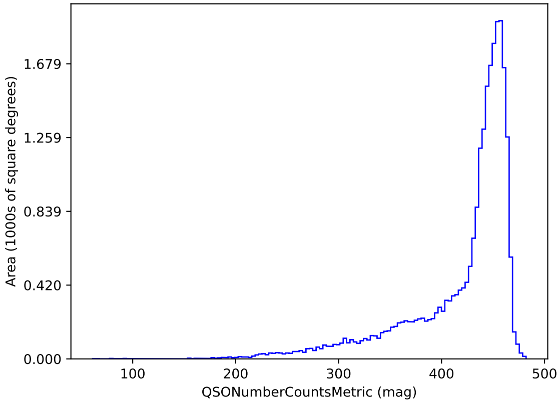
smc_lmc_v3.3_10yrs g band and non-DD: QSONumberCountsMetric
