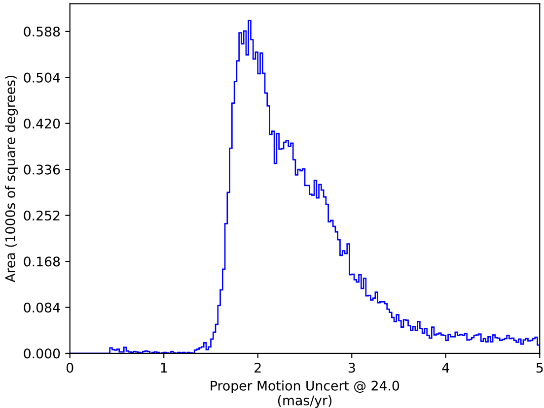
smc_lmc_v3.3_10yrs : Proper Motion Uncert @ 24.0
