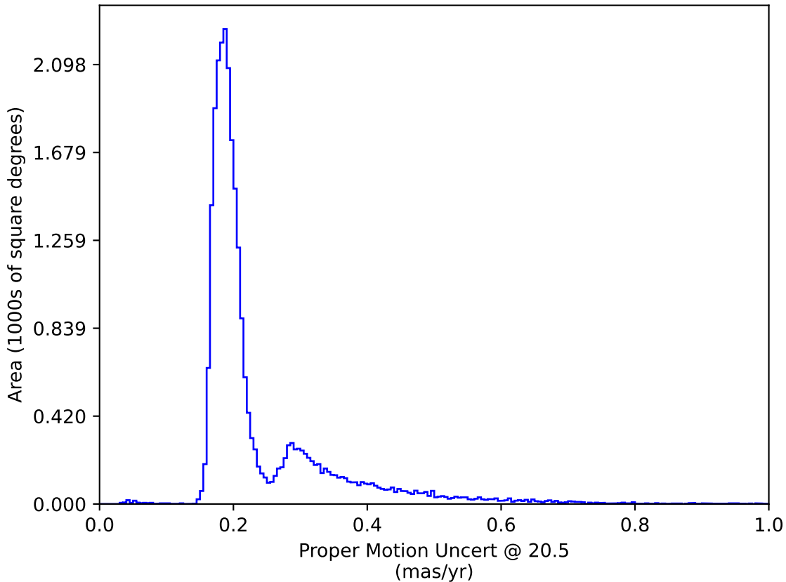
smc_lmc_v3.3_10yrs : Proper Motion Uncert @ 20.5
