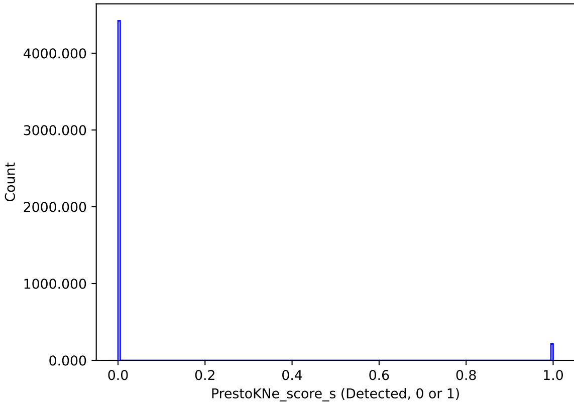
smc_lmc_v3.3_10yrs : PrestoKNe_score_s
