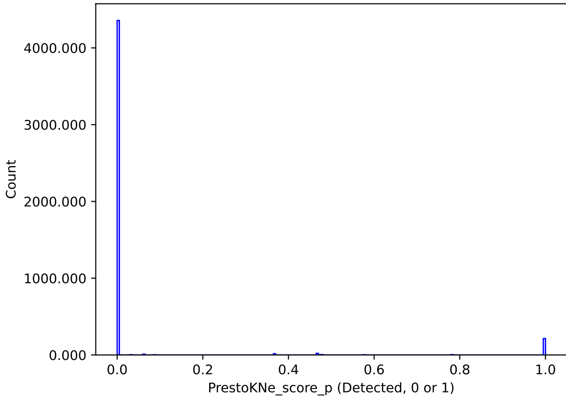
smc_lmc_v3.3_10yrs : PrestoKNe_score_p
