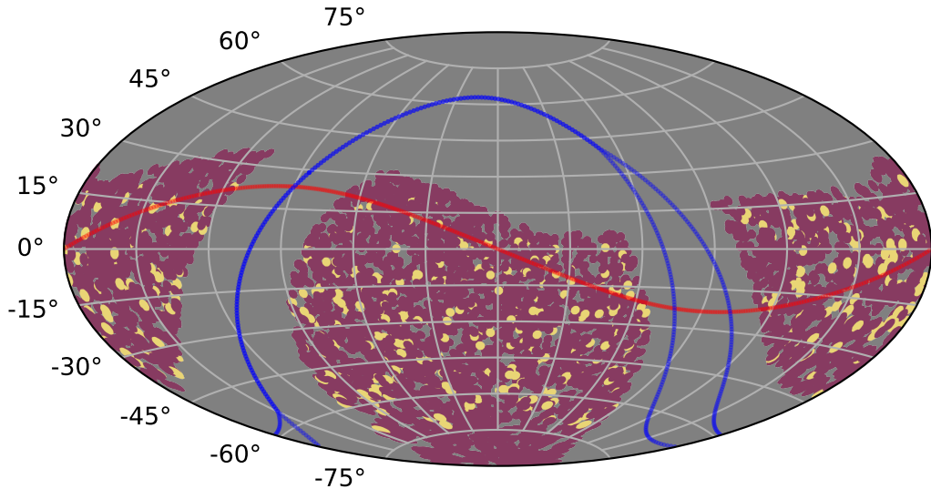
smc_lmc_v3.3_10yrs : PrestoKNe_presto_color_detect
