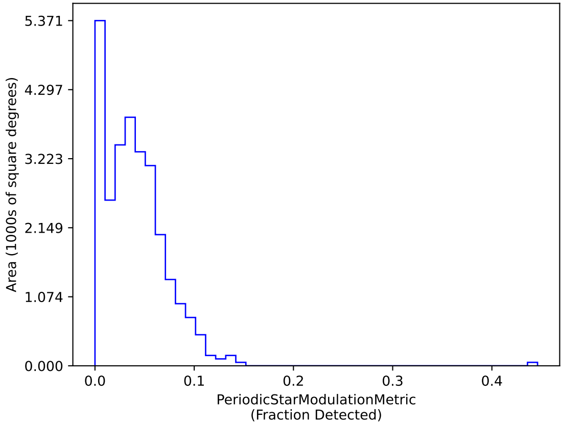
smc_lmc_v3.3_10yrs dm 21 interval 30 RRC Year 1-2: PeriodicStarModulationMetric
