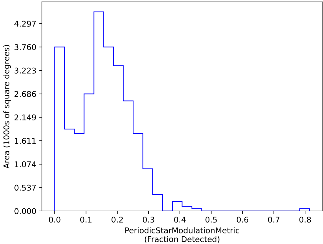
smc_Imc_v3.3_10yrs dm 20 interval 30 RRC Year 1-2: PeriodicStarModulationMetric
