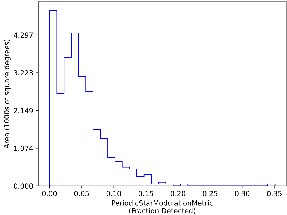
smc_Imc_v3.3_10yrs dm 20 interval 15 RRC Year 1-2: PeriodicStarModulationMetric
