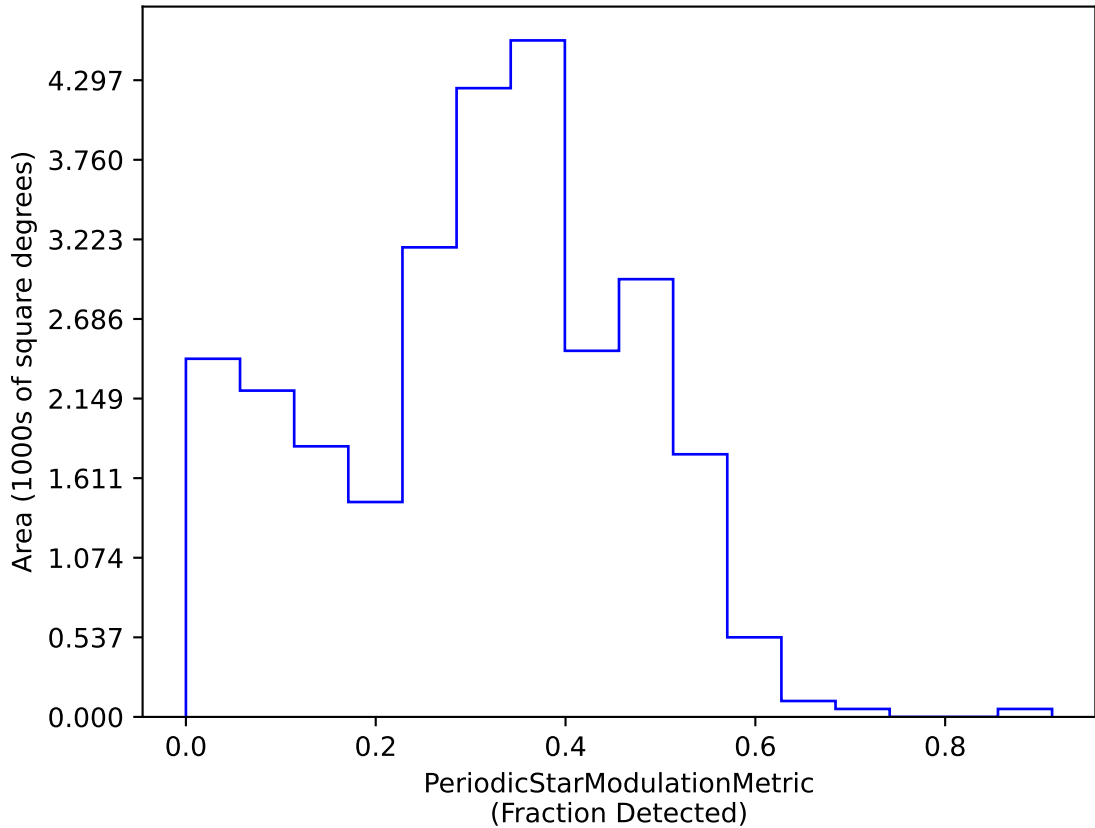
smc_Imc_v3.3_10yrs dm 19 interval 30 RRc Year 1-2: PeriodicStarModulationMetric
