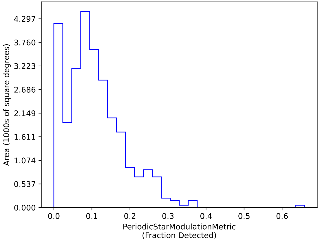
smc_lmc_v3.3_10yrs dm 19 interval 15 RRC Year 1-2: PeriodicStarModulationMetric
