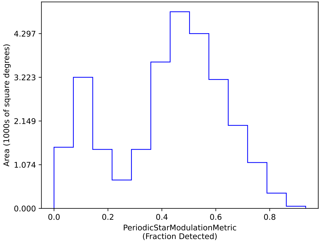
smc_lmc_v3.3_10yrs dm 18 interval 30 RRc Year 1-2: PeriodicStarModulationMetric
