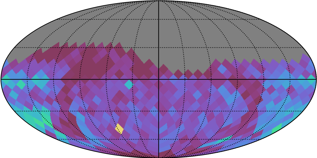
smc_lmc_v3.3_10yrs dm 18 interval 15 RRc Year 1-2: PeriodicStarModulationMetric
