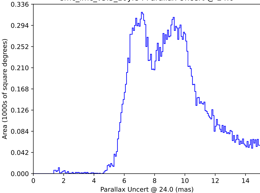
smc_lmc_v3.3_10yrs : Parallax Uncert @ 24.0
