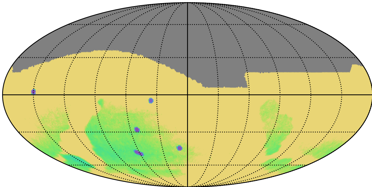
smc_lmc_v3.3_10yrs : Parallax Uncert @ 22.4
