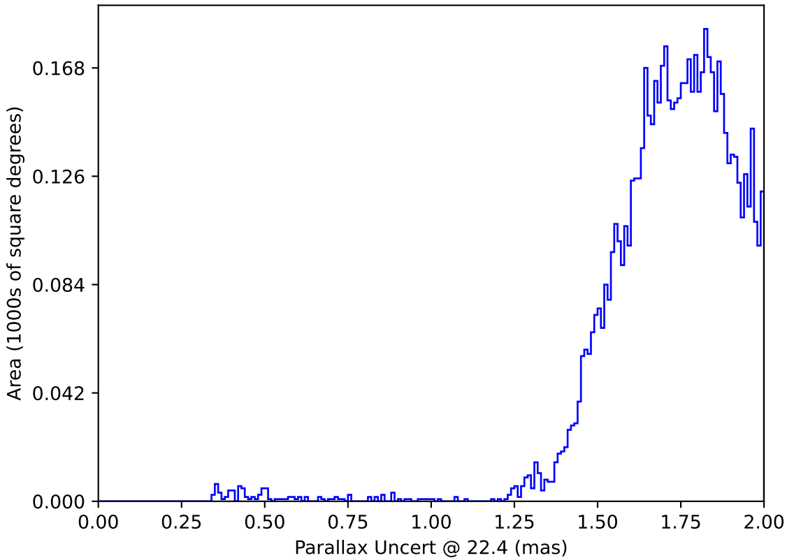
smc_lmc_v3.3_10yrs : Parallax Uncert @ 22.4
