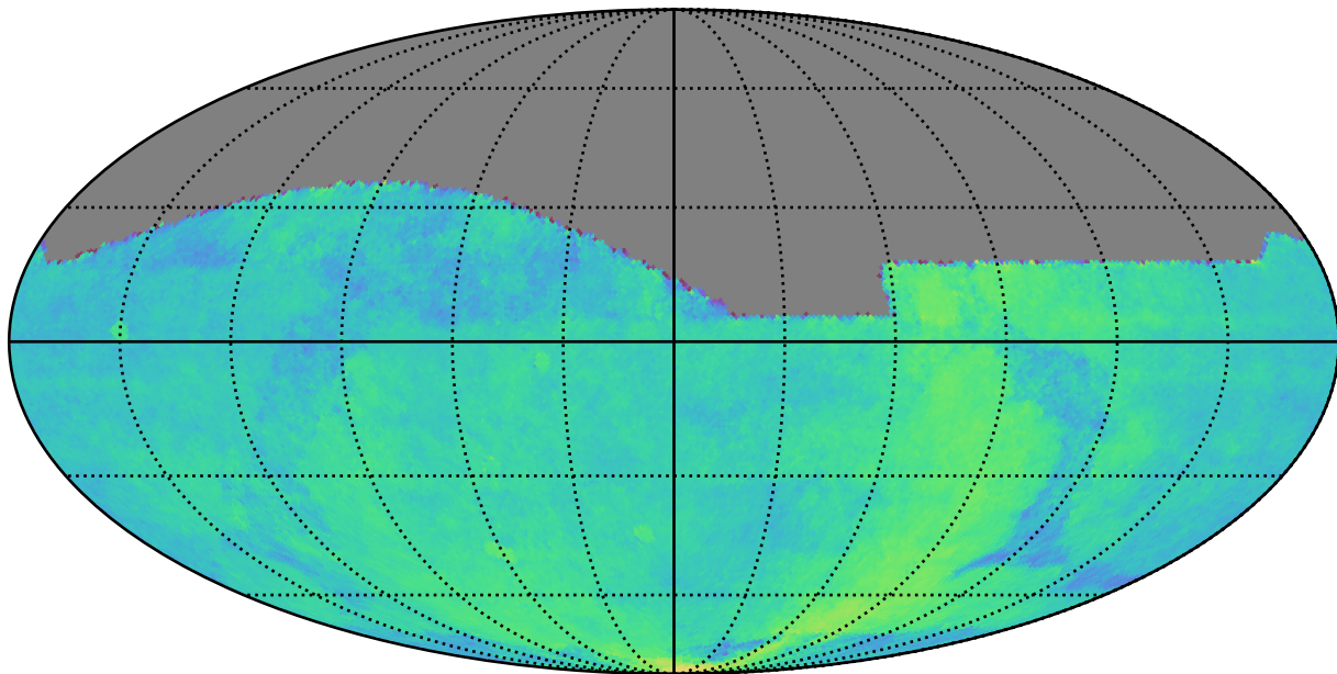
smc_lmc_v3.3_10yrs : Parallax Coverage @ 24.0
