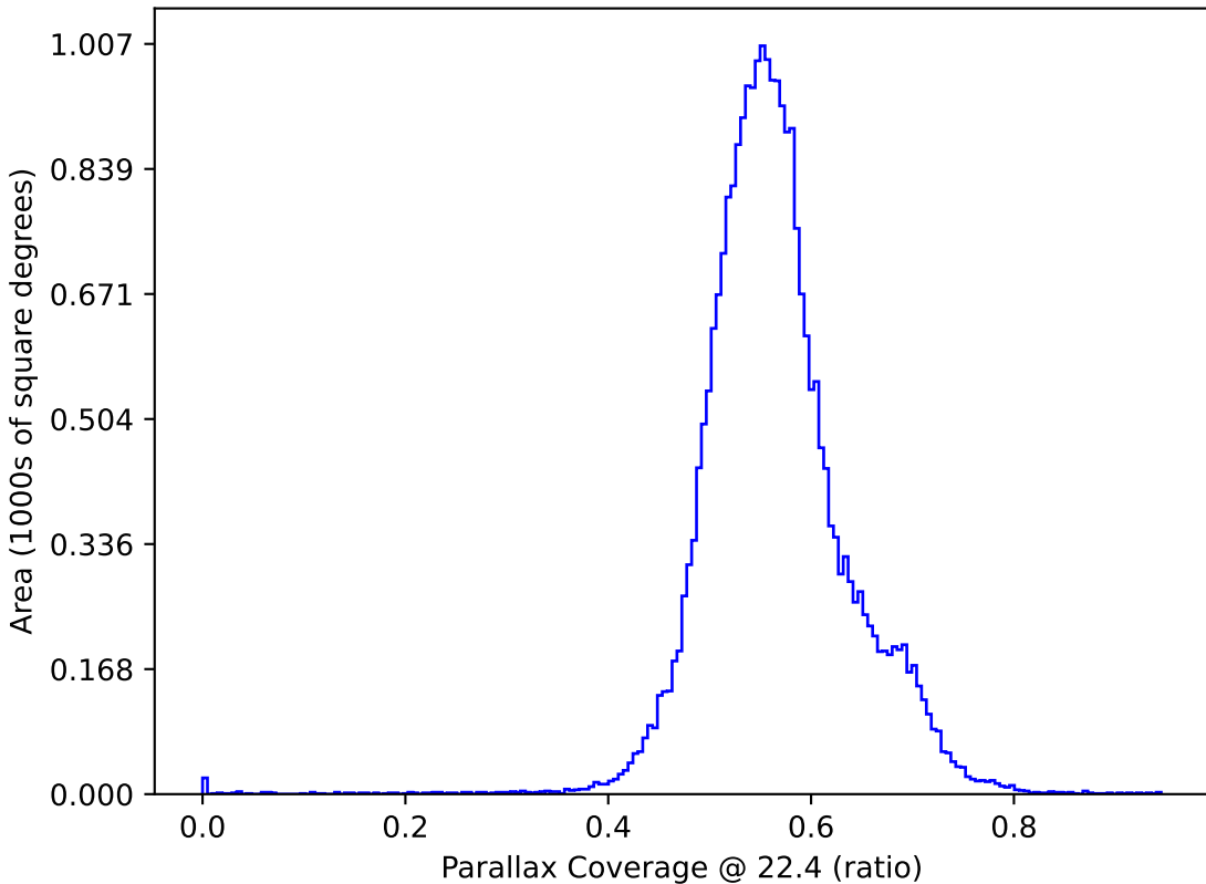
smc_lmc_v3.3_10yrs : Parallax Coverage @ 22.4
