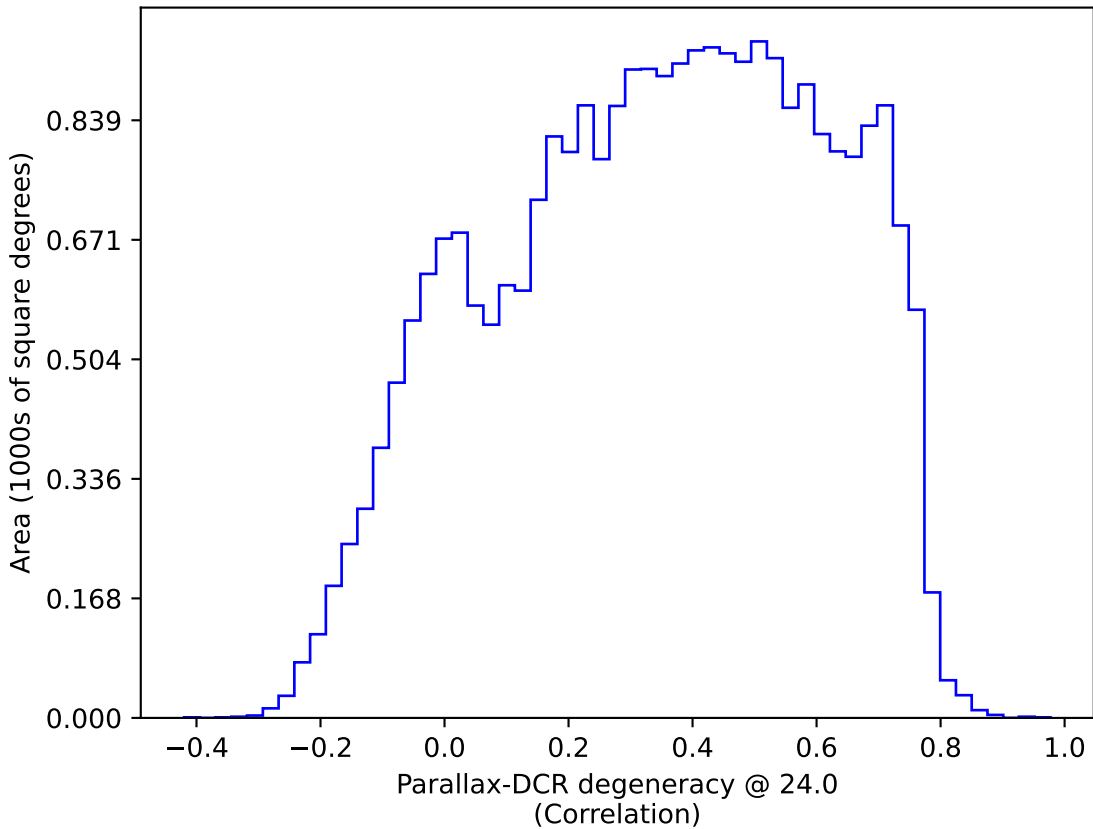
smc_lmc_v3.3_10yrs : Parallax-DCR degeneracy @ 24.0
