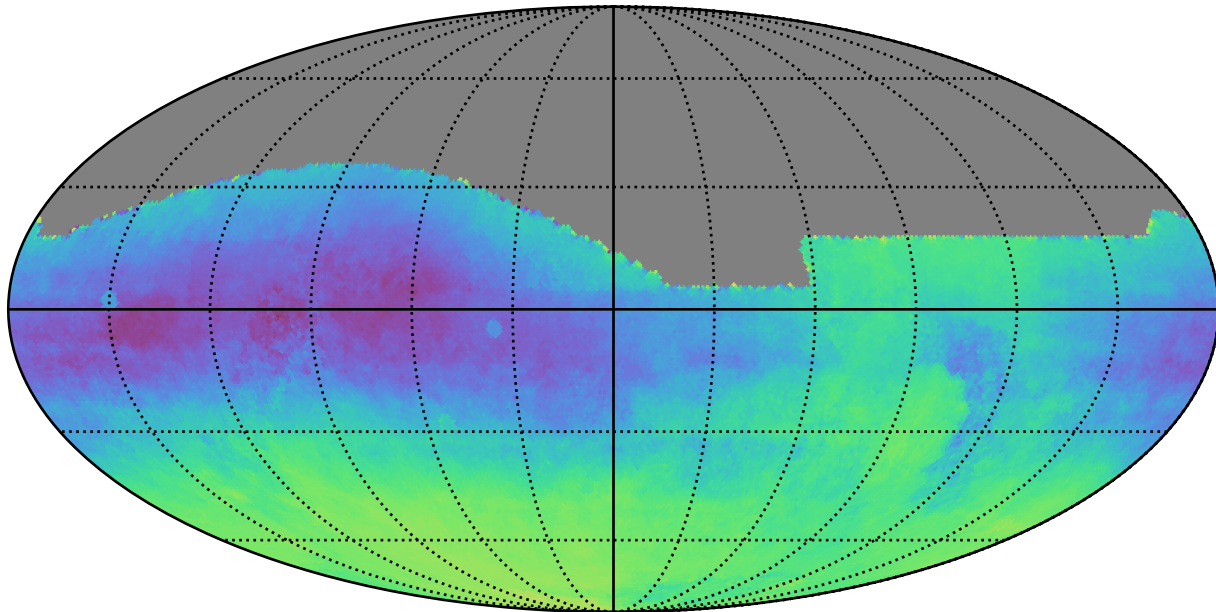
smc_lmc_v3.3_10yrs : Parallax-DCR degeneracy @ 22.4
