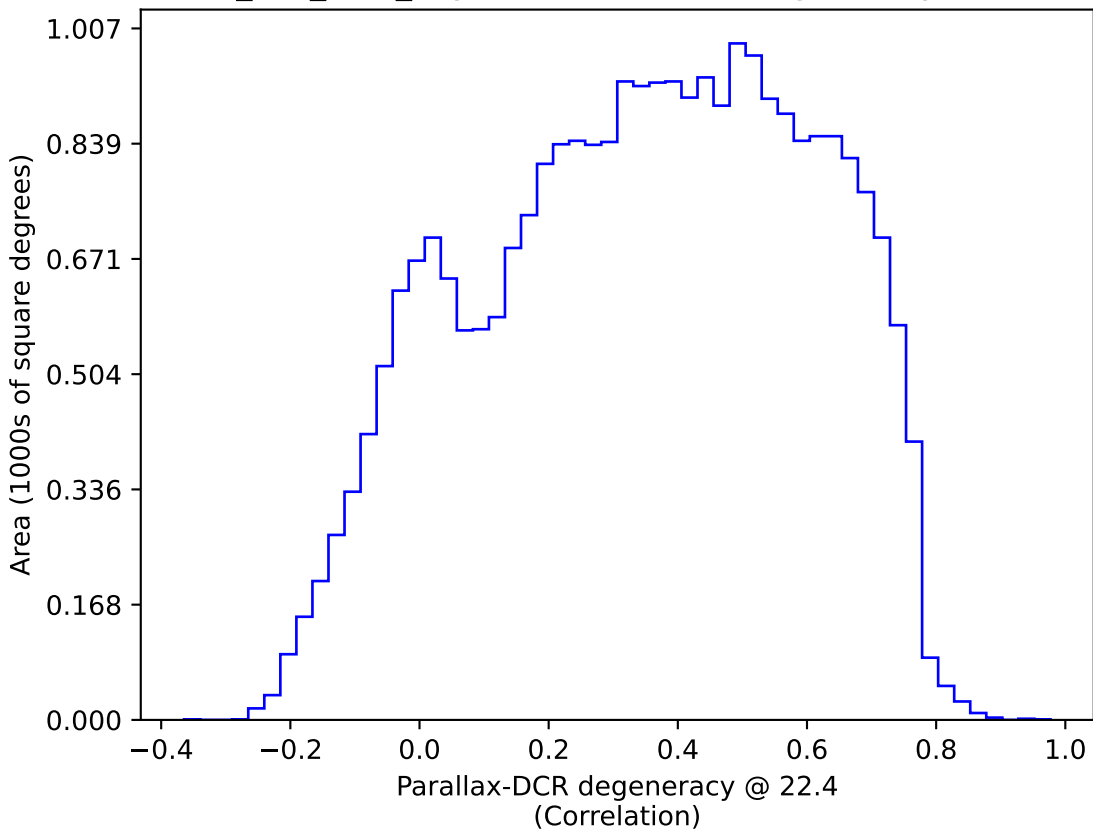
smc_lmc_v3.3_10yrs : Parallax-DCR degeneracy @ 22.4
