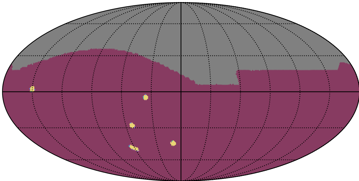
smc_lmc_v3.3_10yrs : NumberOfQuickRevisits
