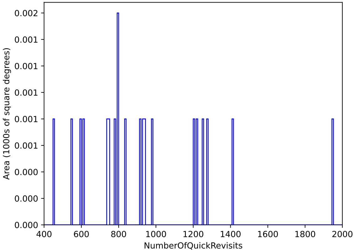
smc_Imc_v3.3_10yrs : NumberOfQuickRevisits
