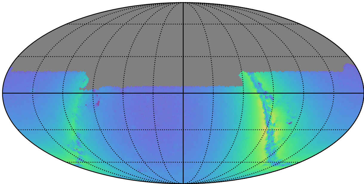
smc_lmc_v3.3_10yrs u: Nstars_no_crowding
